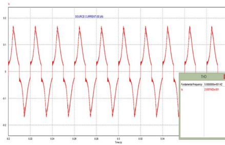
Fig. 9. Total Harmonic Distortion of input current using THD tool in PSIM Simulation
