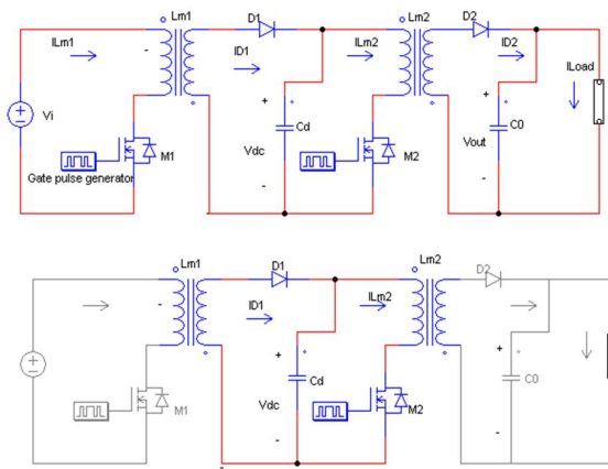
Fig. 2. Derivation of proposed circuit from cascaded flyback converters
