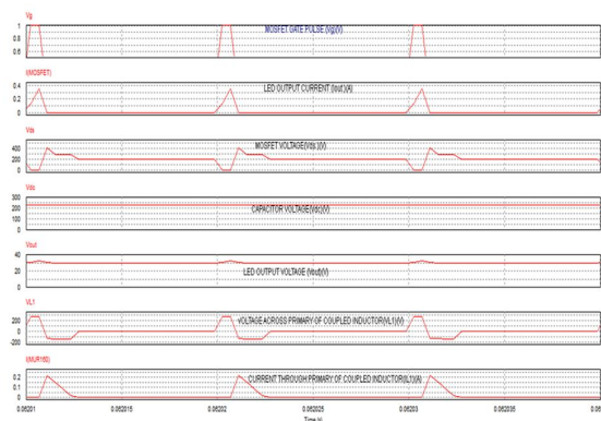
Fig. 8. PSIM Simulation Waveforms of Proposed pulsating current LED driver
