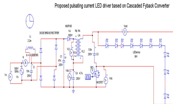
Fig. 7. PSIM Simulation Model of Proposed pulsating current LED driver
