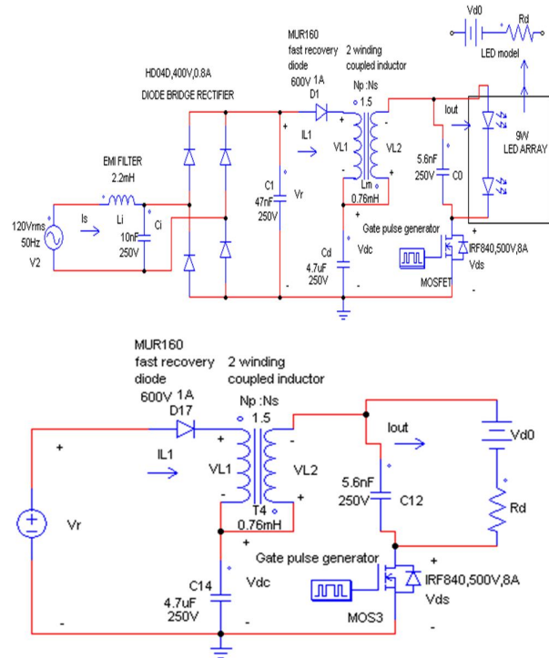
Fig. 3. Proposed pulsating current LED and Equivalent circuit with rectified voltage source
