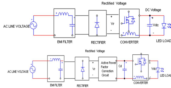
Fig.1. Typical AC/DC single stage and two-stage LED driver
