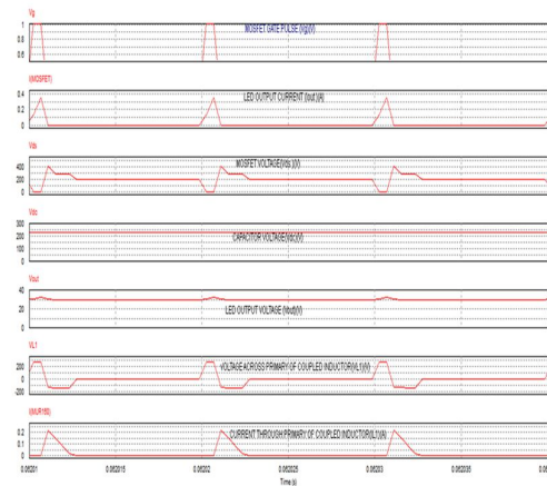
Fig. 5. Key Waveforms of the Proposed pulsating current LED driver
