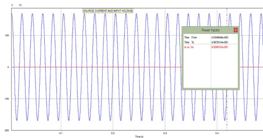
Fig. 10. Power Factor of input side using PF tool in PSIM Simulation
