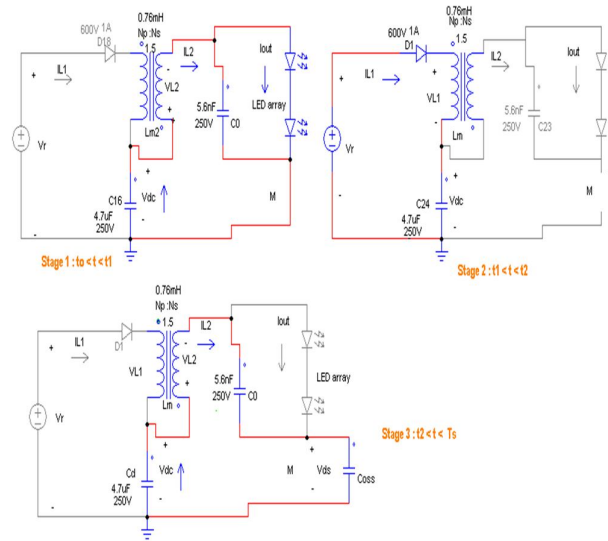
Fig. 4. Operating stages of the proposed LED driver
